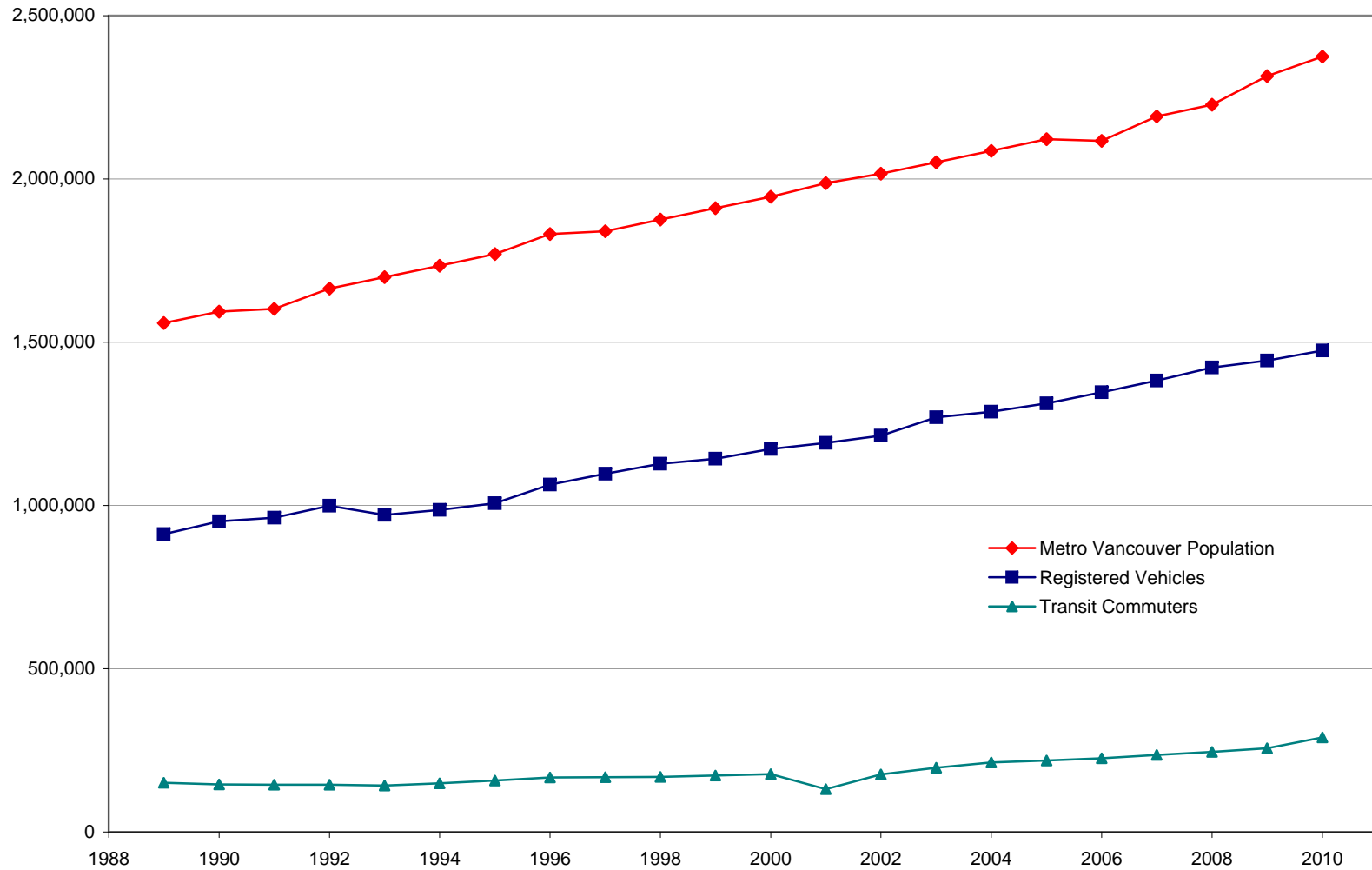
Daily Metro Vancouver Transit Commuters and Registered Vehicles for Metro Vancouver Population
